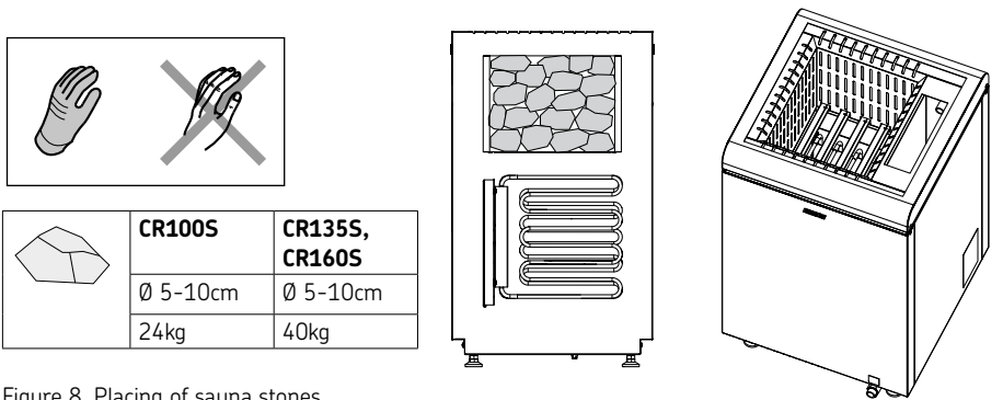
Figure 8. Placing of sauna stones
