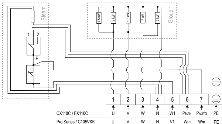
Figure 5. Wiring diagram CR100S
