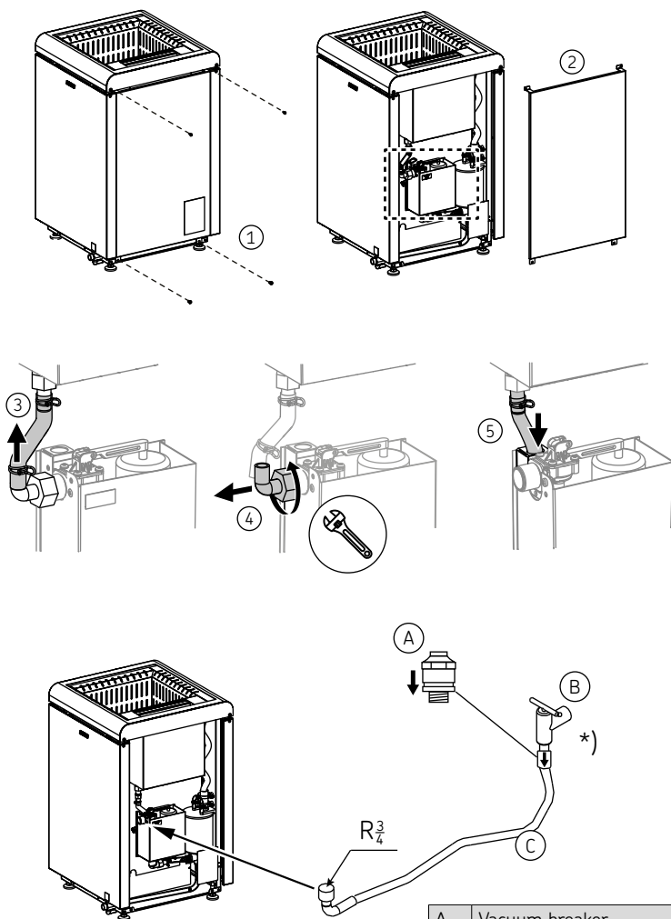
Figure 7. Automatic water supply
