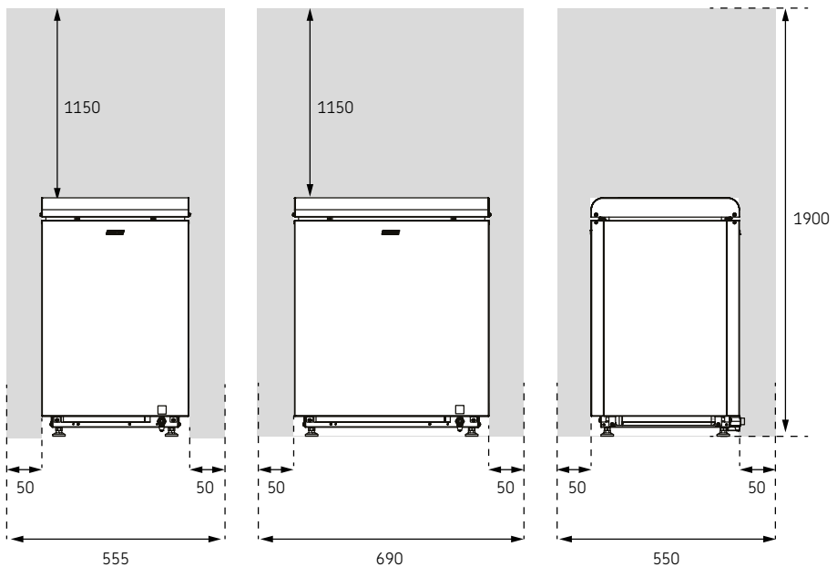
Figure 1. Safety distances
