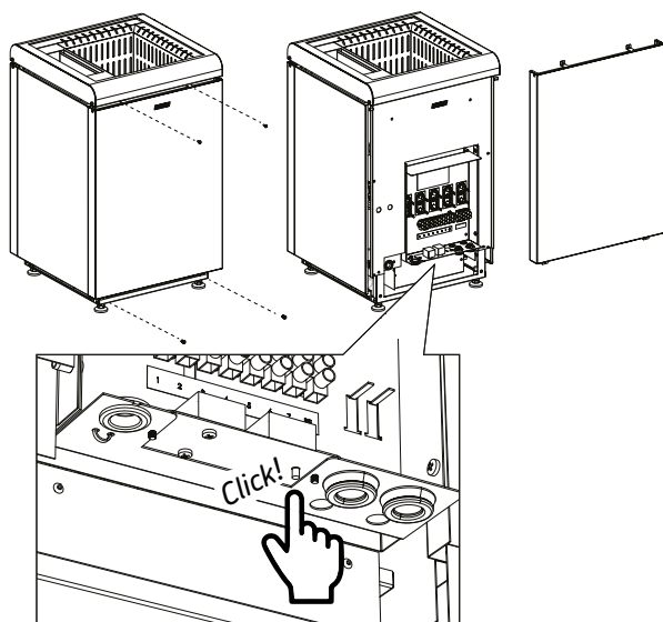
Figure 13. Steamer overheat protector reset
