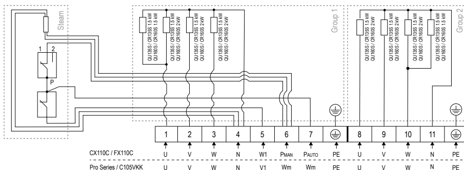
Figure 6a. Wiring diagram CR135S, CR160S
